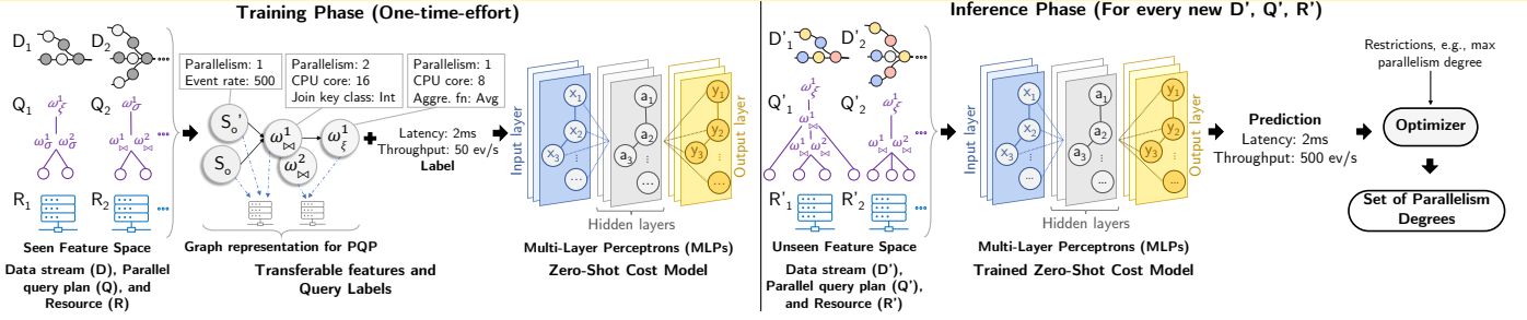
Fig. 2: Overview of ZEROTUNE for cost prediction that can be used in the parallelism tuning task. We train ZEROTUNE (see left fig.) using transferable features of a wide range of streaming workloads with different parallelism degrees. Once the model is trained, it can be used in the inference phase (see right fig.) to accurately estimate the cost of unseen parallelism degrees without requiring costly retraining of the model. Based on the costs, an optimizer is used to select the parallelism degree that has the minimum cost.
